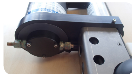
SeaFET connected to MicroCAT pumped flow path
